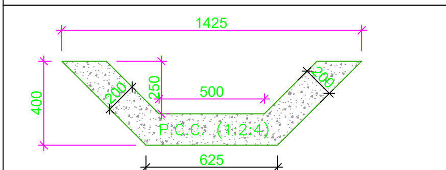
NUMERATION DETAIL OF LEACHATE COLLECTION TRENCH FOR 160mm HDPE PIPE
