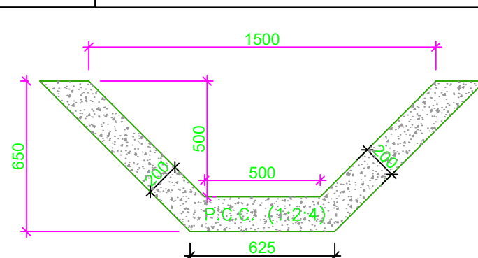
NUMERATION DETAIL OF LEACHATE COLLECTION TRENCH FOR 225 HDPE PIPE
