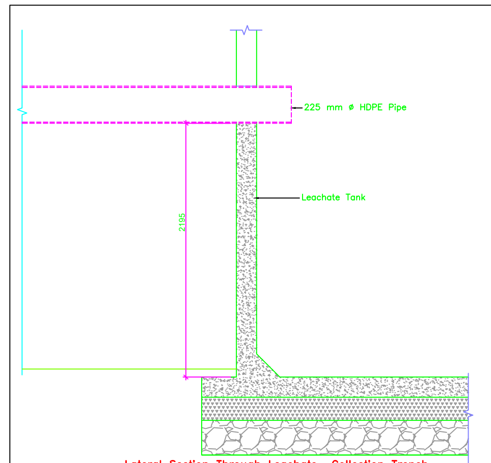
Lateral Section Through Leachate Collection Trench
