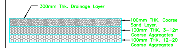
DETAILS OF DRAINAGE LAYER
