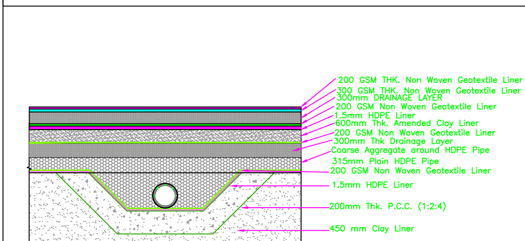
160mm \varnothing Lateral Perforated HDPE Pipe laid in P.C.C. Trench for Leachate Collection
