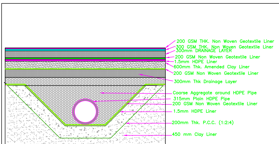
225mm \varnothing Main Header HDPE Pipe laid in P.C.C. Trench for Leachate Collection
