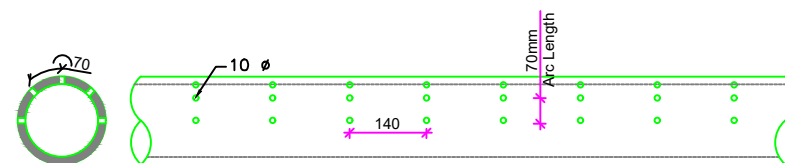
Detail of Perforations for 160mm HDPE Pipe for Leachate Collection
